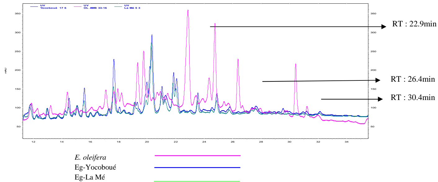
Figure 1: Comparison between sensitive materials ( E. guineensis Yocoboué, and La Mé) and not-attacked ( E. oleifera ). RT: Retention Time.
