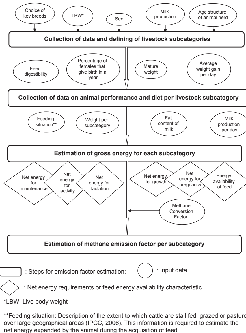
Figure 1 Flow chart of methodology used for enteric methane EF estimate: IPCC (2006).
