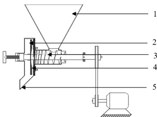
Fig. 10. Design of almond mill with carborundum stone
