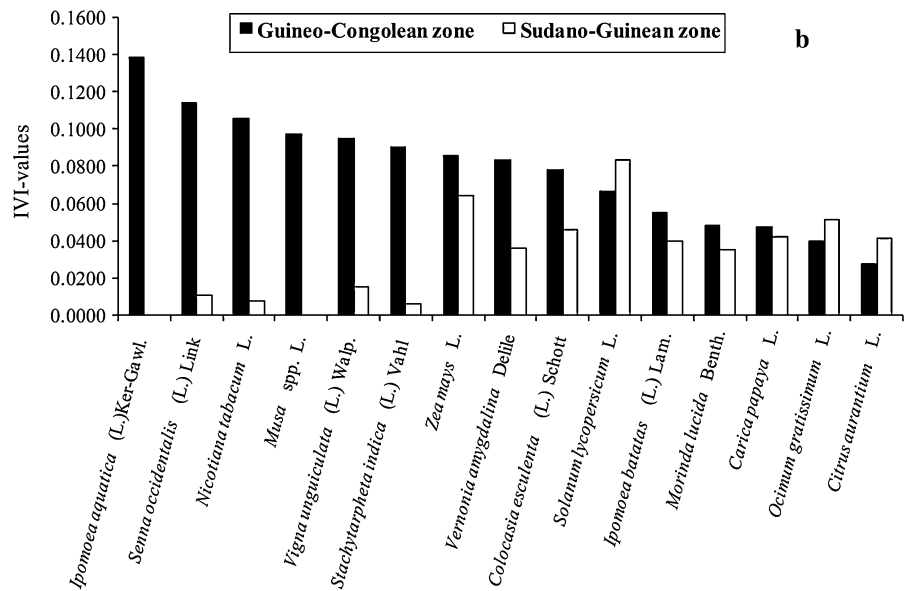
Most important species (species of cluster 5, see table 4)
