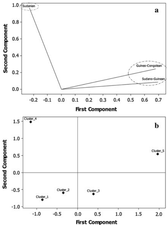
Fig. 6 Principal Components analysis of the IVI-values of home garden species according to climatic zones: (a) projection of the IVI-values for each climatic zone in the system axis defined by the principal components; (b) projection of the 5 clusters of home gardens species in the system axis defined by the climatic zones IVI-values
