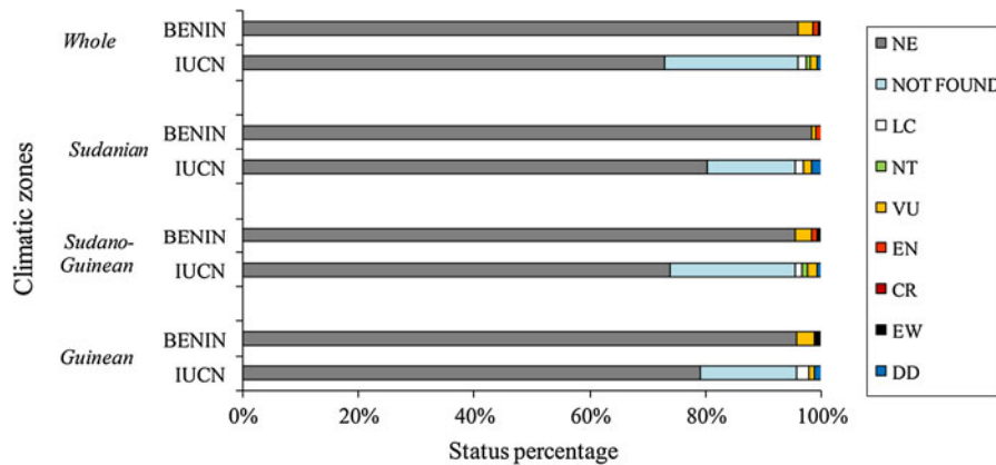
Fig. 8 Home gardens species conservation status according to climatic zones. Threatened status: LC least concern, NT near threatened, VU vulnerable, EN endangered, CR critically endangered, EW extinct in the wild, DD data deficient, NE not evaluated, NF not found
