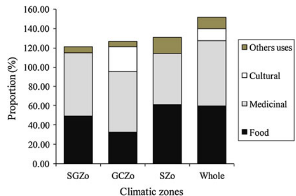
Fig. 3 Uses categories of home gardens species according to the climatic zones. GCZo Guineo-Congolean Zone, SGZo Sudano-Guinean Zone, SZo Sudanian Zone. Other uses = Fodder + ornamental + timber + fence
