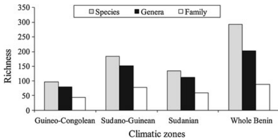
Fig. 2 Species, genera and family richness of home gardens according to the climatic zones
