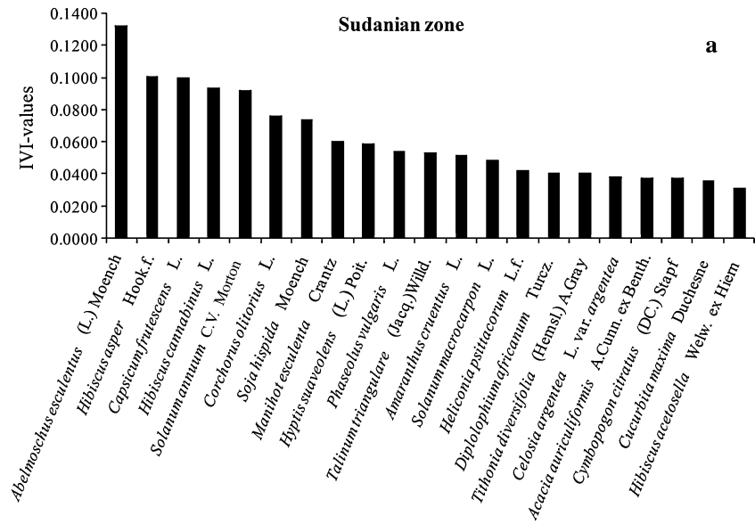
Most important species (species of cluster 4, see table 4)
