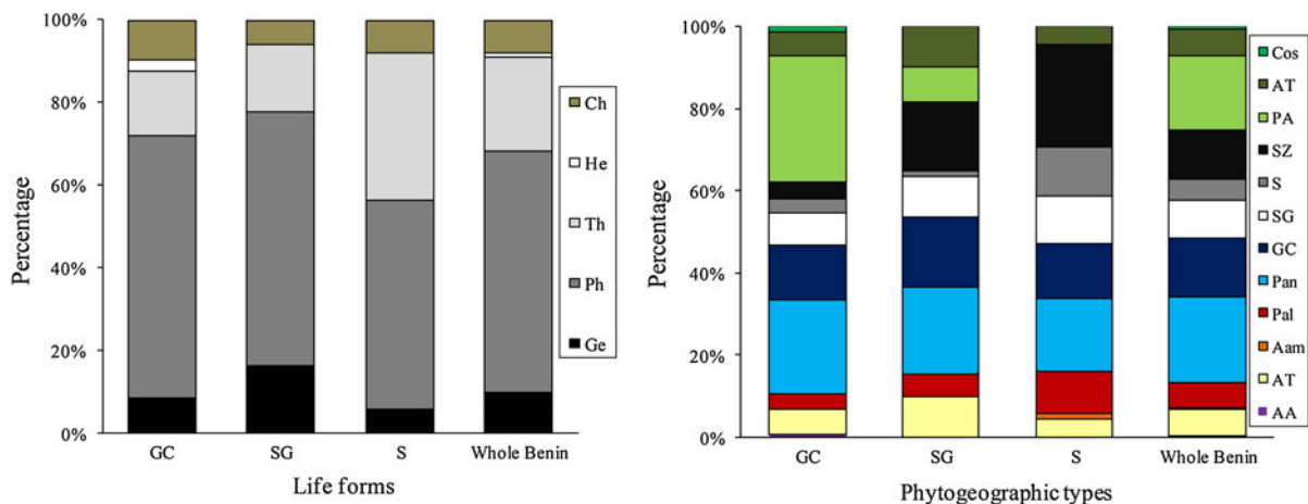
Fig. 4 Life forms types (a) and phylogeographic types (b) of home gardens species. Climatic zones: GCZo Guineo-Congolese Zone, SGZo Sudano-Guinean Zone, SZo Sudanian Zone. Life forms: Ch Chamephytes, He Hemicryptophytes, Th Therophytes, Ph Phanerophytes, Gc Geophytes. Phylogeographic
