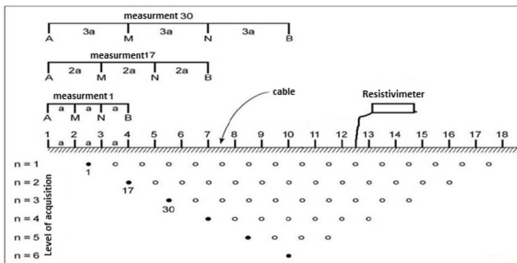
Fig. 3. Arrangement of the electrodes for a 2D acquisition and a sequence of measurement for a Wenner alpha device ([29])
