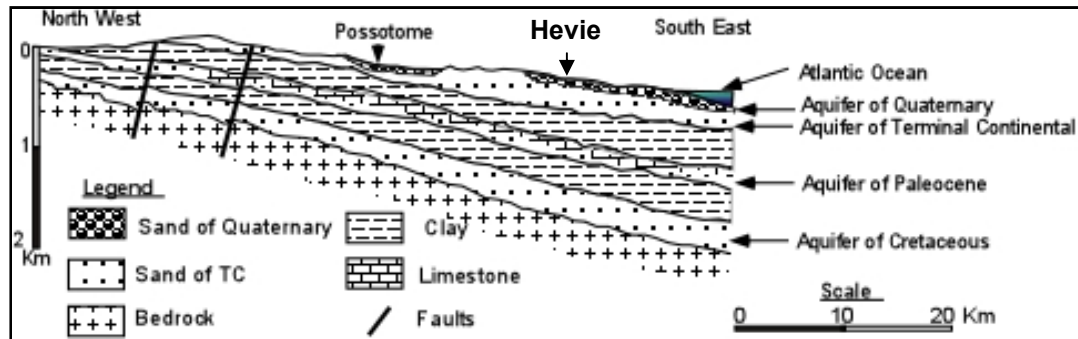
Fig. 2. Hydrogeological section of coastal sedimentary basin of Benin (Source: [25] modified in [3])
