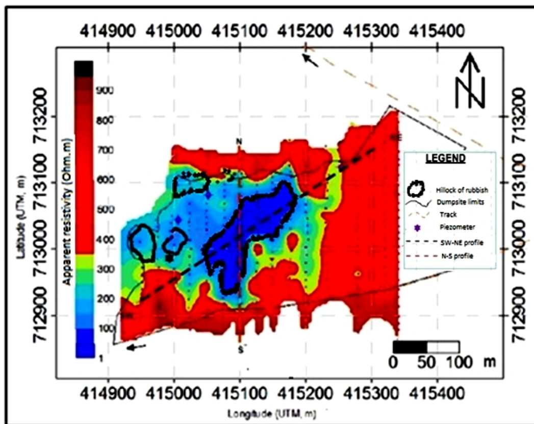
Fig. 7. Localization of the ERT profiles on the electromagnetic map
