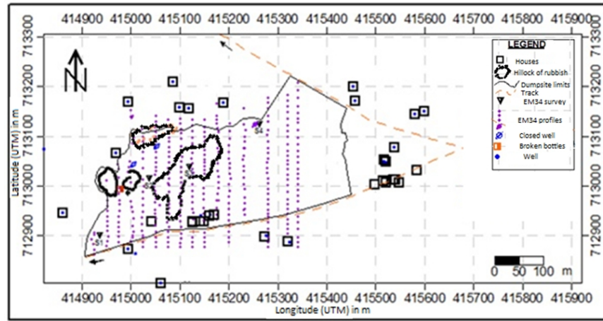
Fig. 4. Chart of the EM34 profiles and electromagnetic surveys distribution on the dumpsite of Hevie
