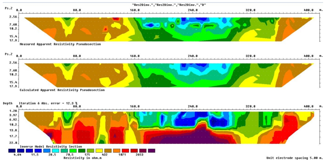
Fig. 8(a). Interpreted ERT section according to the N-S profile
