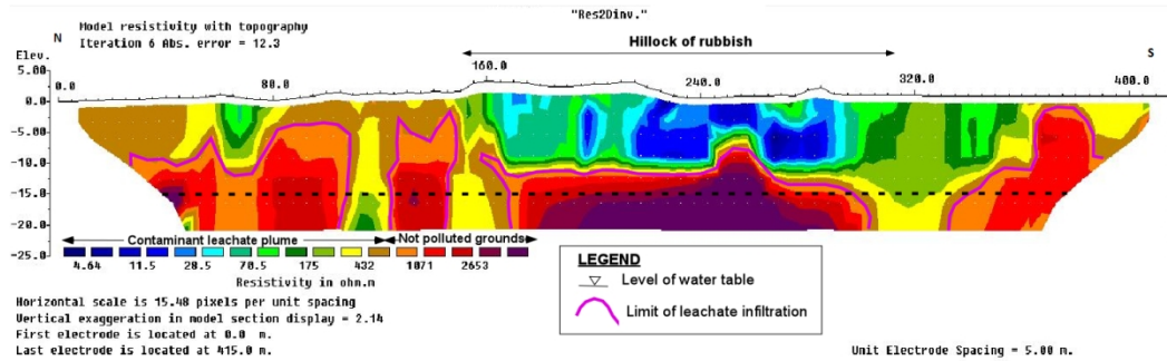
Fig. 9a. ERT N-S section showing the water table – leachate plume contact
