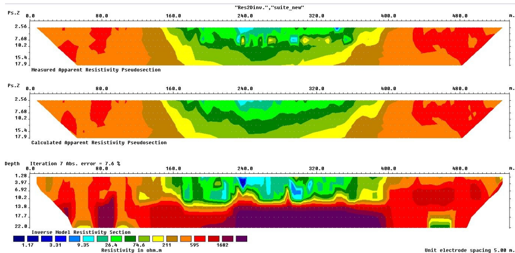
Fig. 8(b). Interpreted ERT section according to the SW-NE profile
