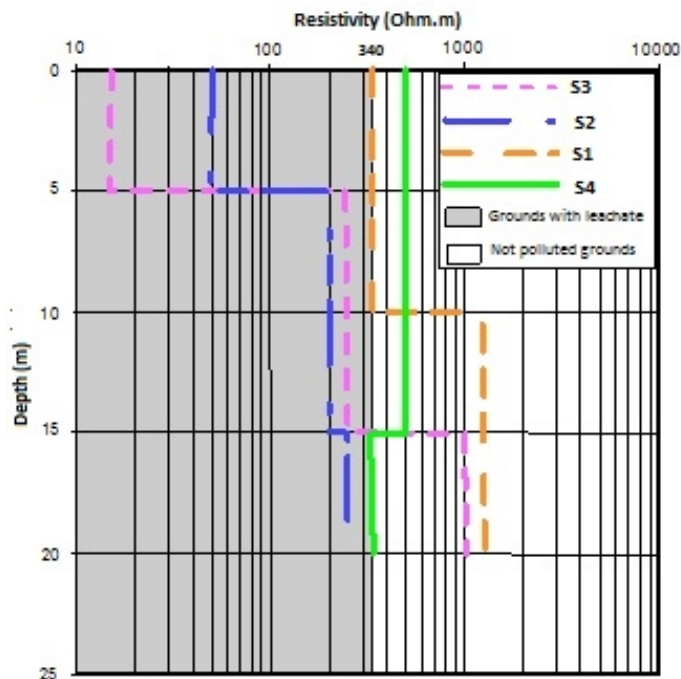
Fig. 6. Logs of surveys EM showing S2-S3 in grounds with leachate plume and S1-S4 in unpolluted grounds
