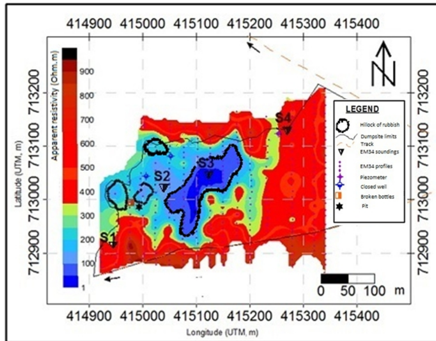
Fig. 5. Map of lateral extension of the leachate at 10m of depth using EM34
